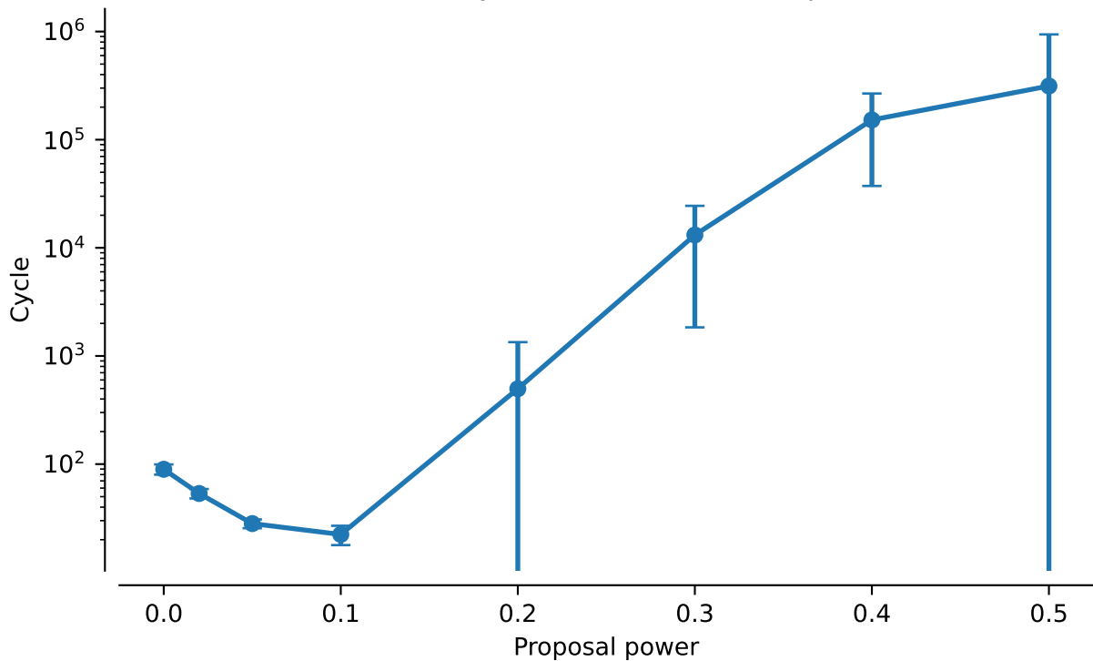
vert.coiii.tw0: NNI Cycles to discover 95% posterior mass
