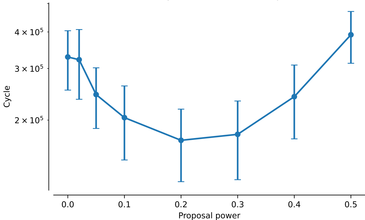
vert.coiii.tw2: NNI Cycles to discover 95% posterior mass
