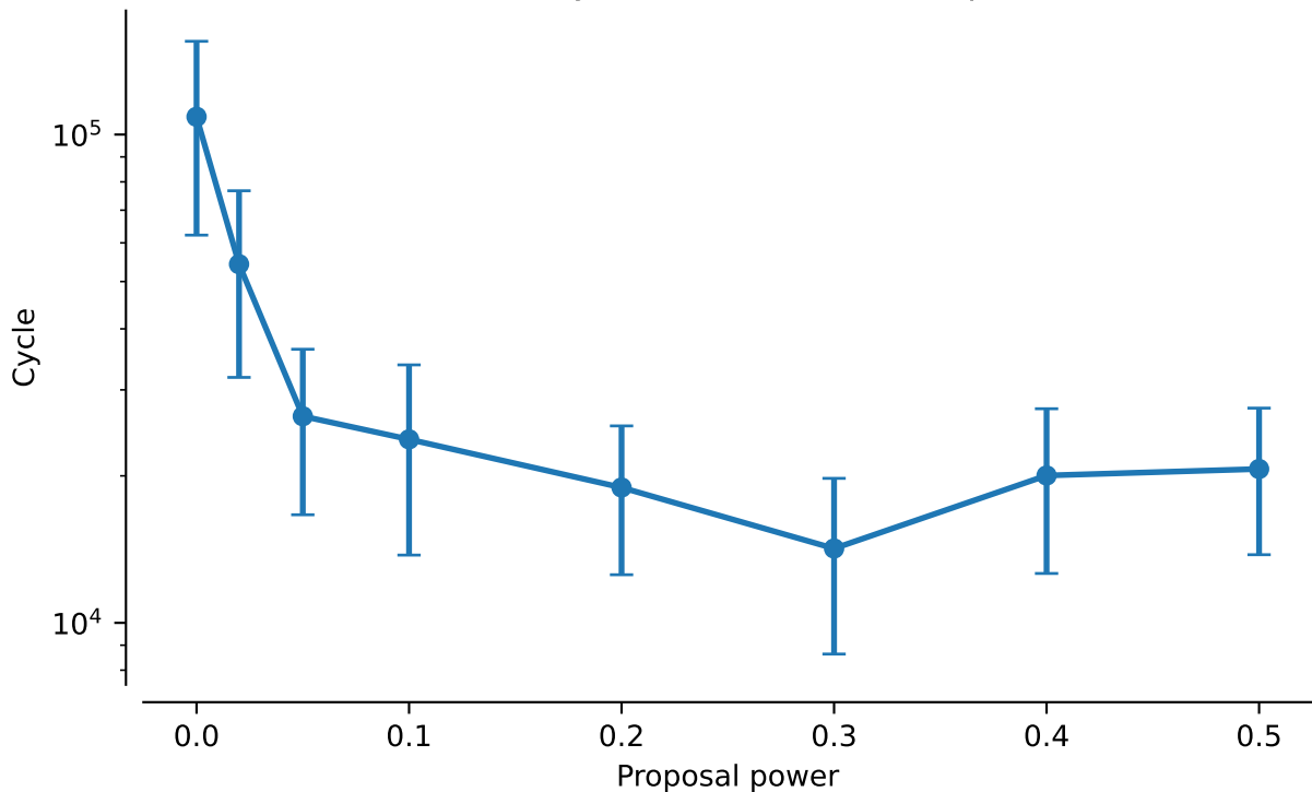
vert.nd1.tw5: NNI Cycles to discover 95% posterior mass
