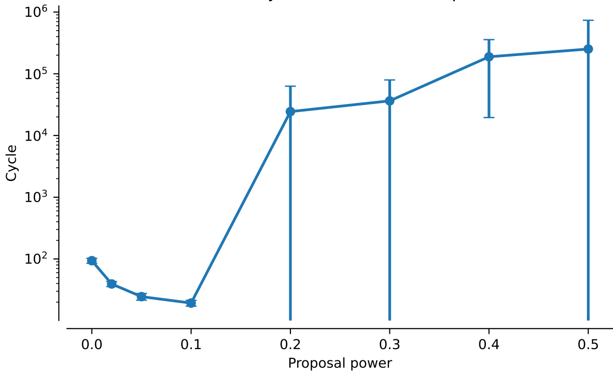
vert.nd2.tw0: NNI Cycles to discover 95% posterior mass
