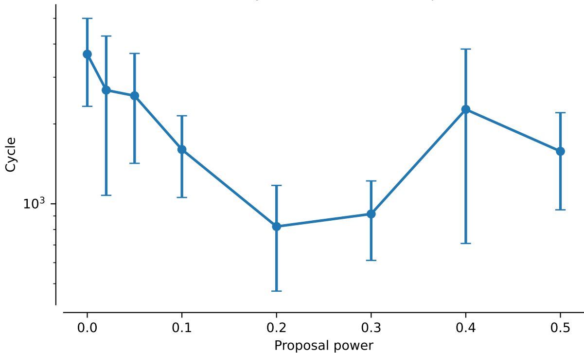
vert.nd2.tw5: NNI Cycles to discover 95% posterior mass
