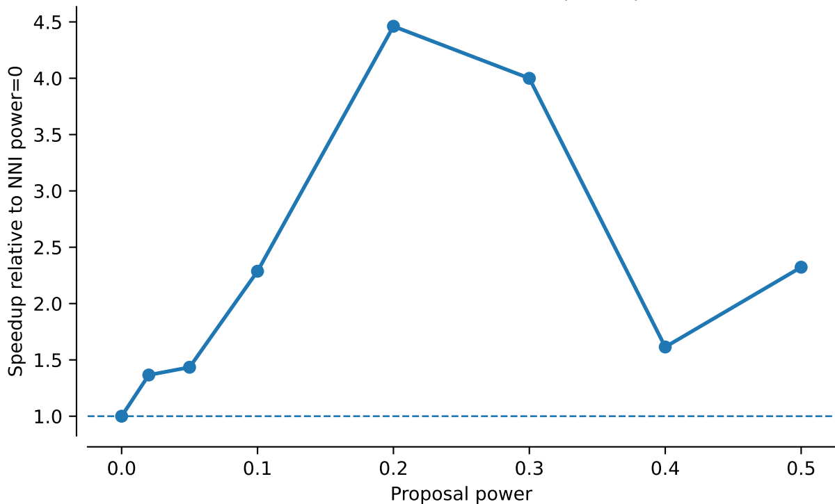
vert.nd2.tw5: NNI tau95 speedup
