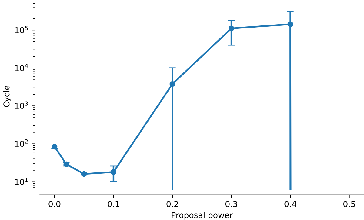
vert.nd4.tw0: NNI Cycles to discover 95% posterior mass
