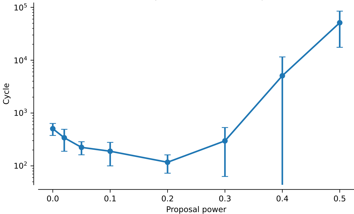
vert.nd4.tw5: NNI Cycles to discover 95% posterior mass
