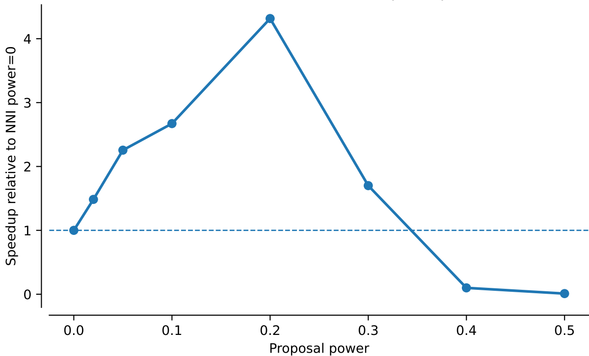
vert.nd4.tw5: NNI tau95 speedup
