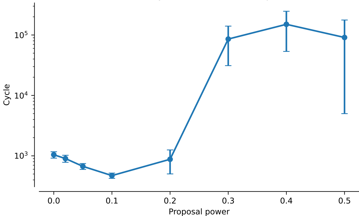
vert.nd4l.tw0: NNI Cycles to discover 95% posterior mass
