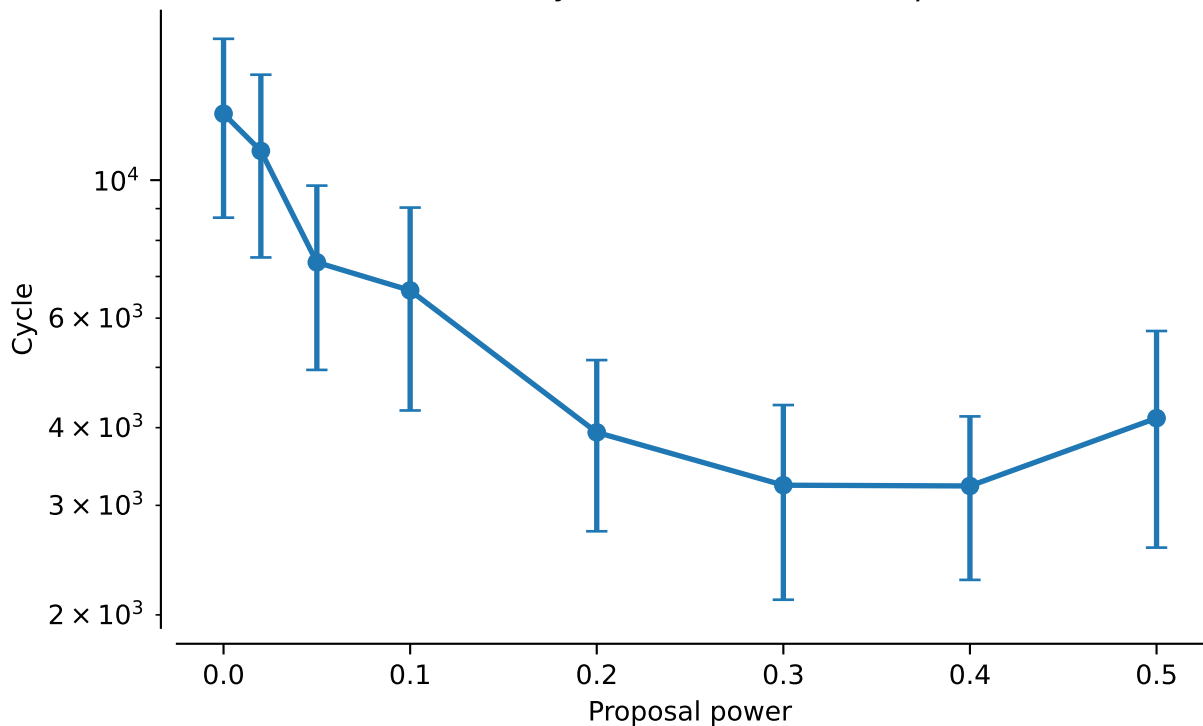
vert.nd4l.tw5: NNI Cycles to discover 95% posterior mass
