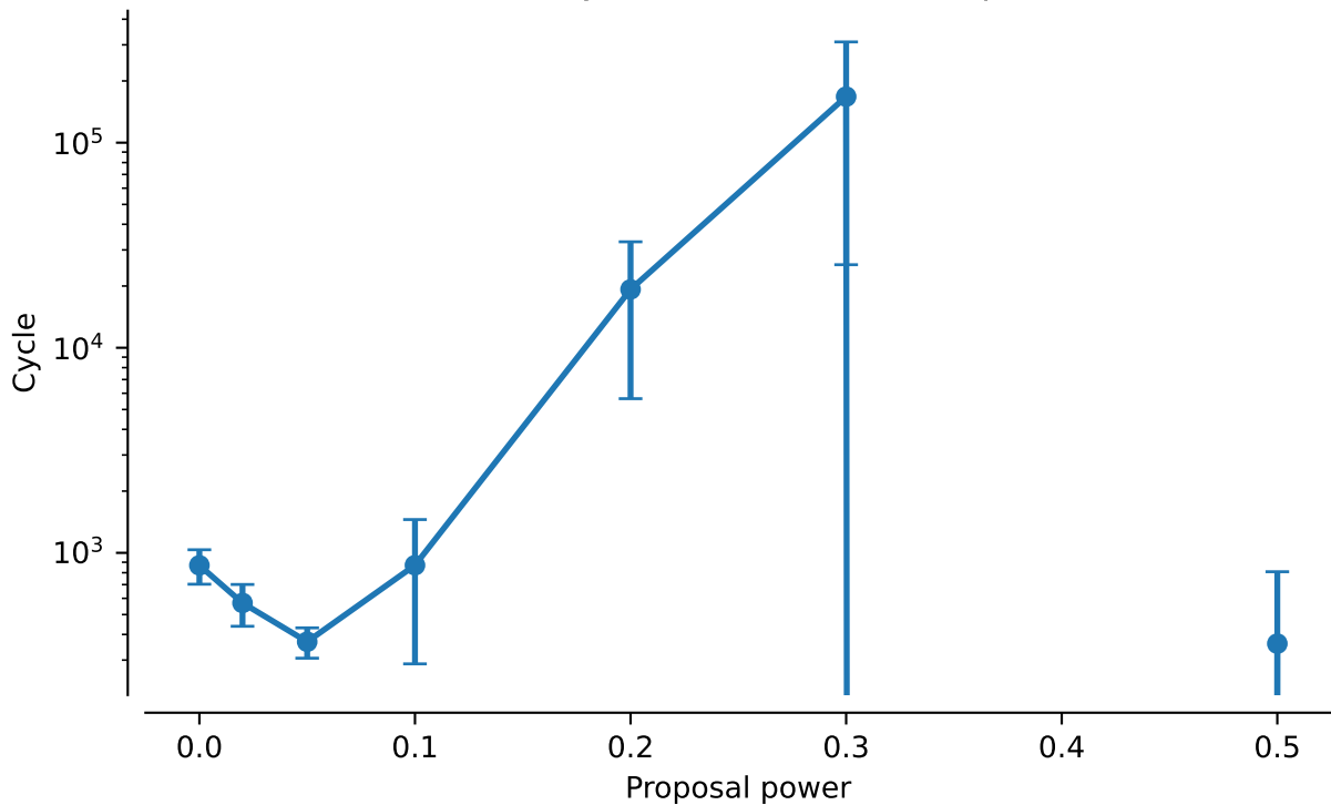
vert.nd6.tw0: NNI Cycles to discover 95% posterior mass
