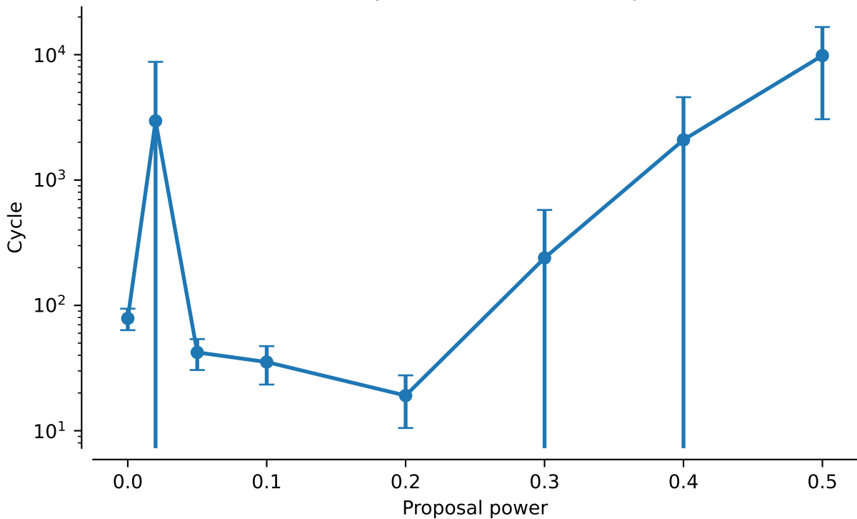
vert.nd6.tw5: NNI Cycles to discover 95% posterior mass
