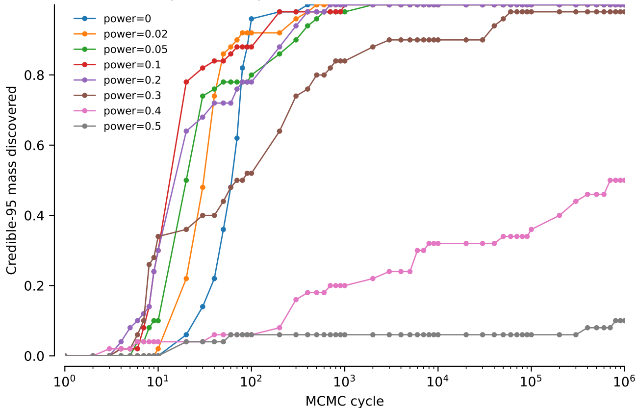
NNI power comparison: Credible-95 mass discovered
