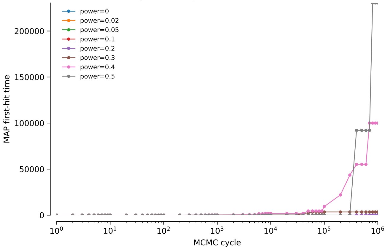
NNI power comparison: MAP first-hit time
