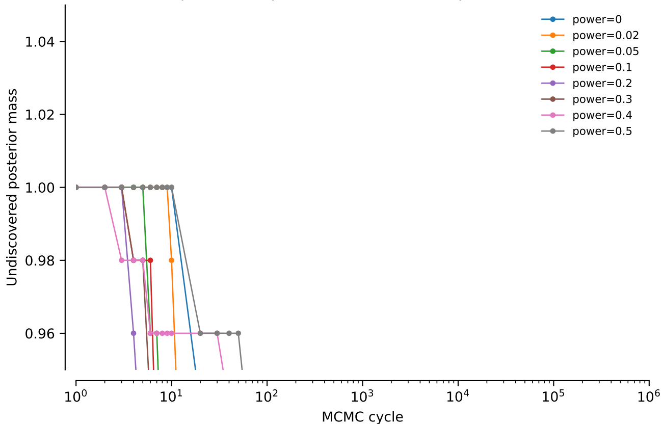
NNI power comparison: Undiscovered posterior mass
