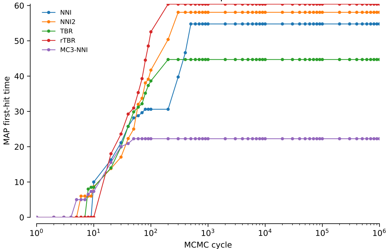
MAP first-hit time: power = 0.02
