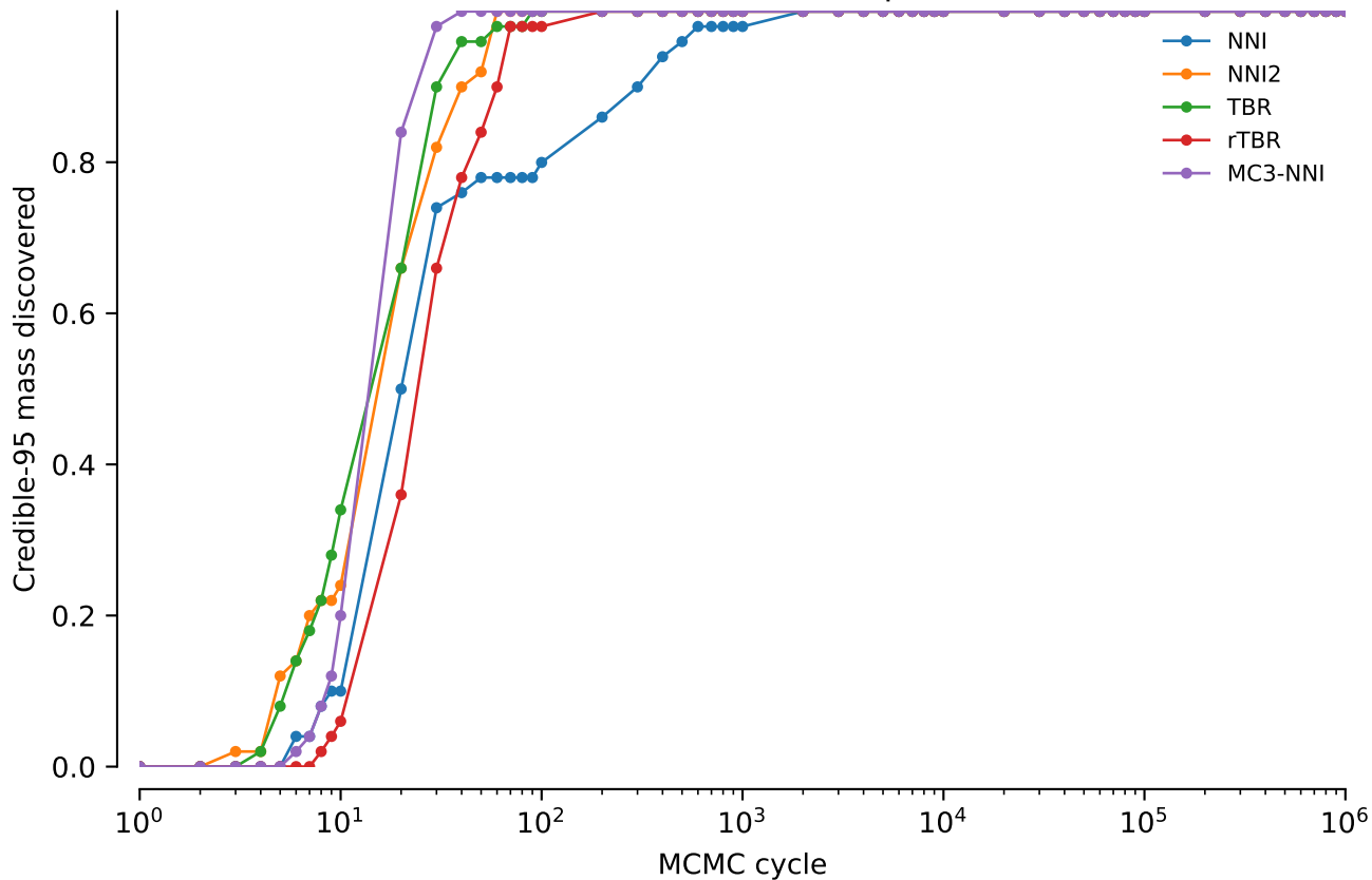
Credible-95 mass discovered: power = 0.05
