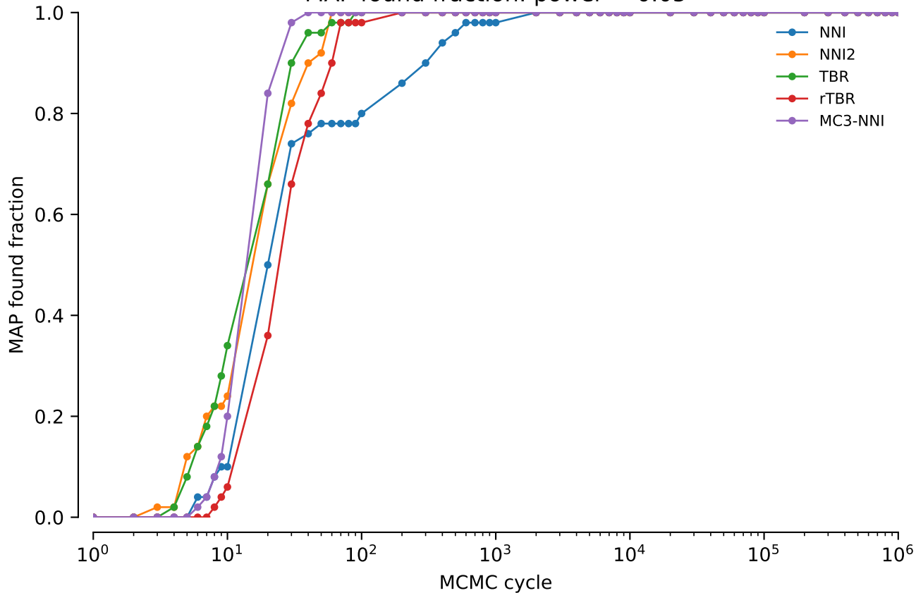
MAP found fraction: power = 0.05
