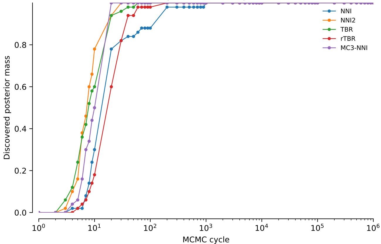
Discovered posterior mass: power = 0.1
