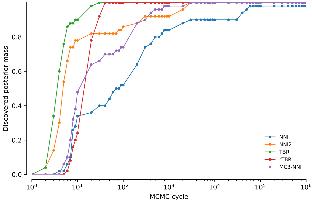
Discovered posterior mass: power = 0.3
