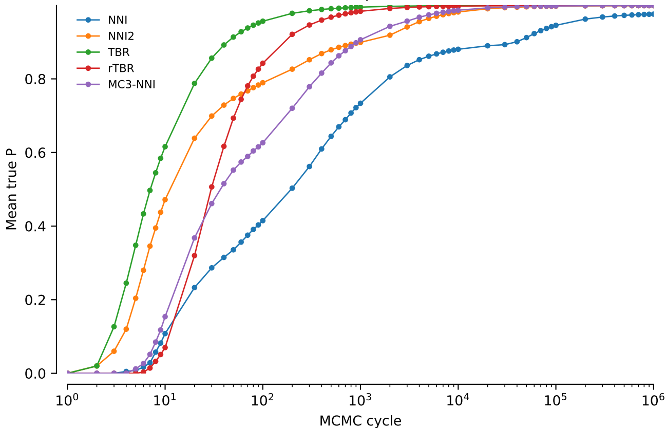
Mean true P: power = 0.3
