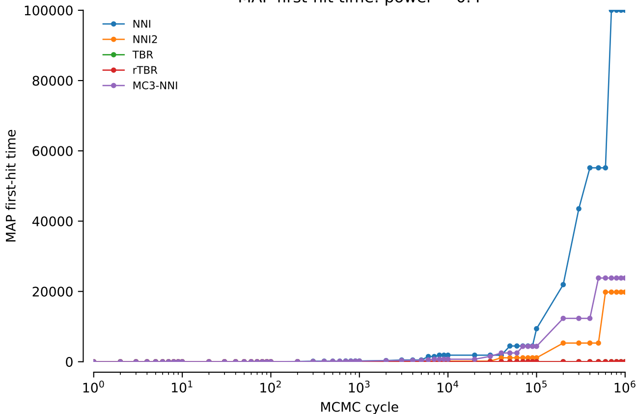
MAP first-hit time: power = 0.4
