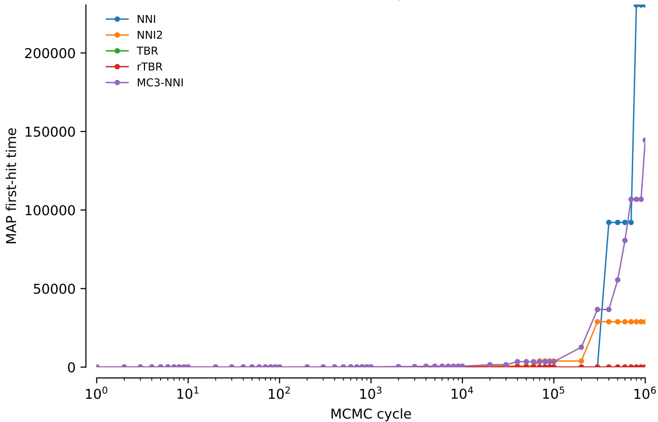
MAP first-hit time: power = 0.5
