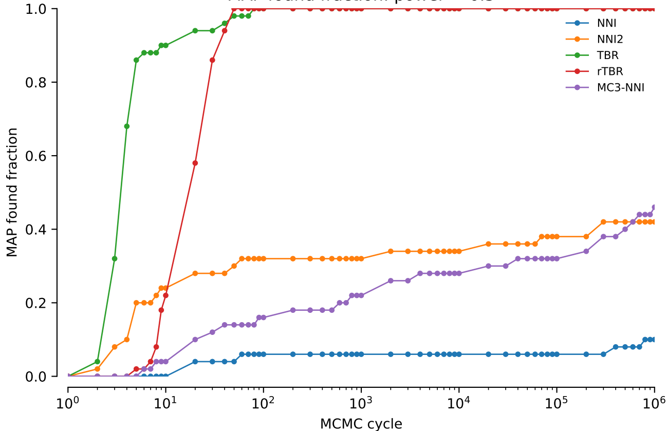
MAP found fraction: power = 0.5
