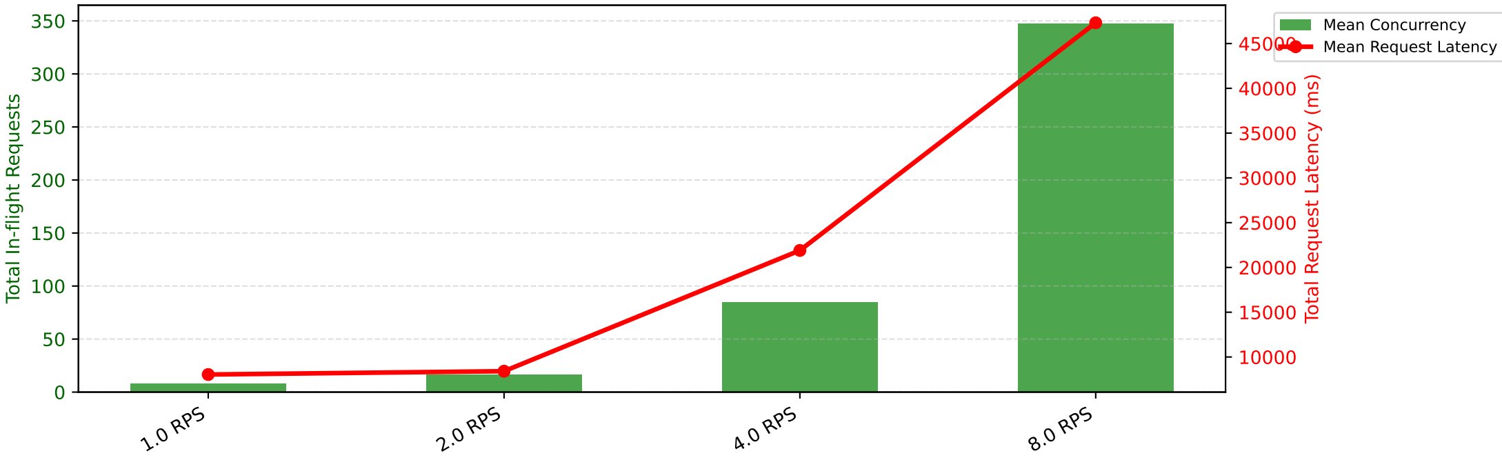
Request Concurrency vs End-to-End Latency Profile
