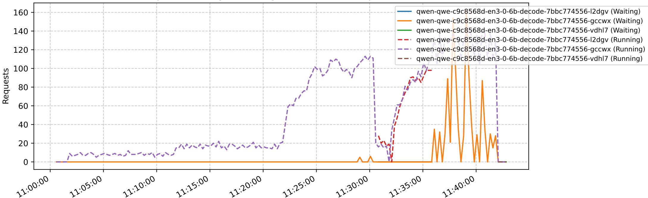
Number of Requests Waiting & Running Over Time (Namespace: wva-bench-test)
