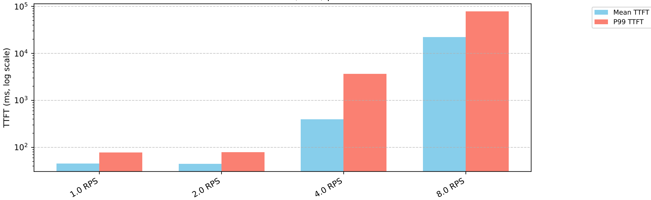
Time To First Token (TTFT) per Run
