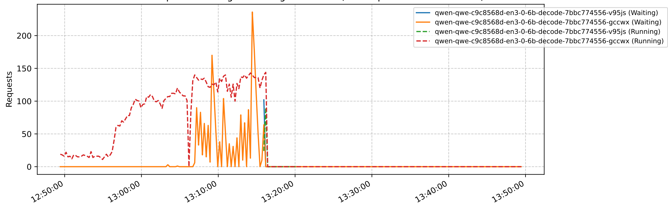
Decode Replica Count &amp; EPP Queue Over Time (Namespace: wva-bench-test)
