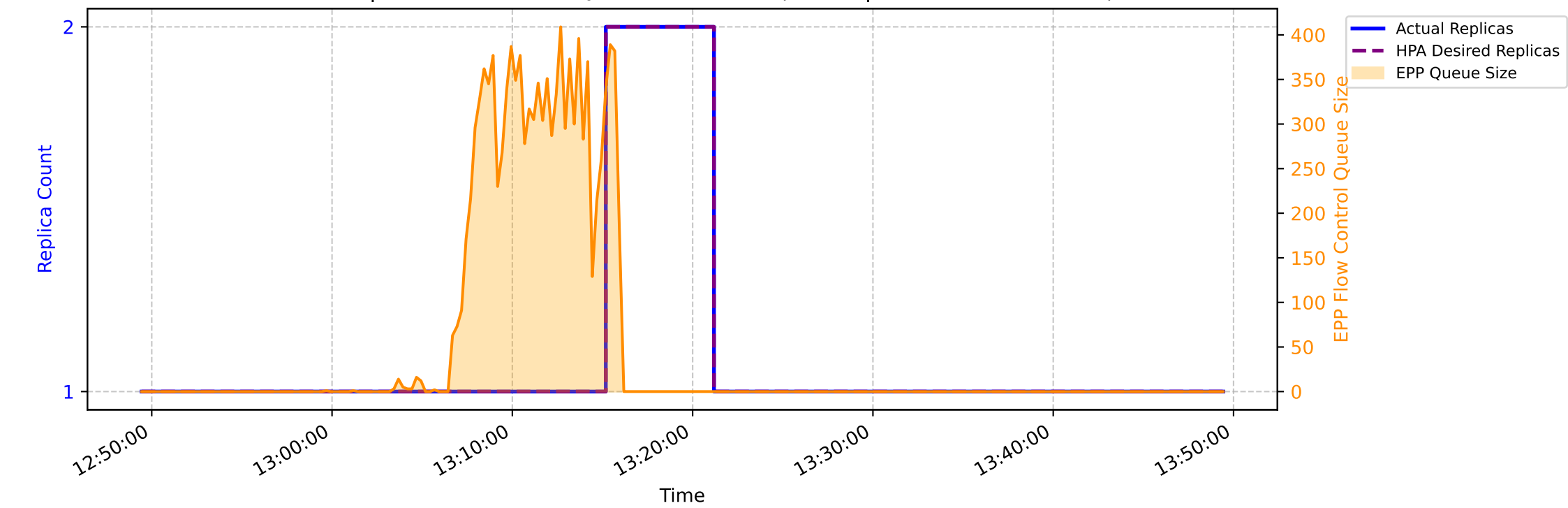
Decode Replica Count &amp; EPP Queue Over Time (Namespace: wva-bench-test)
