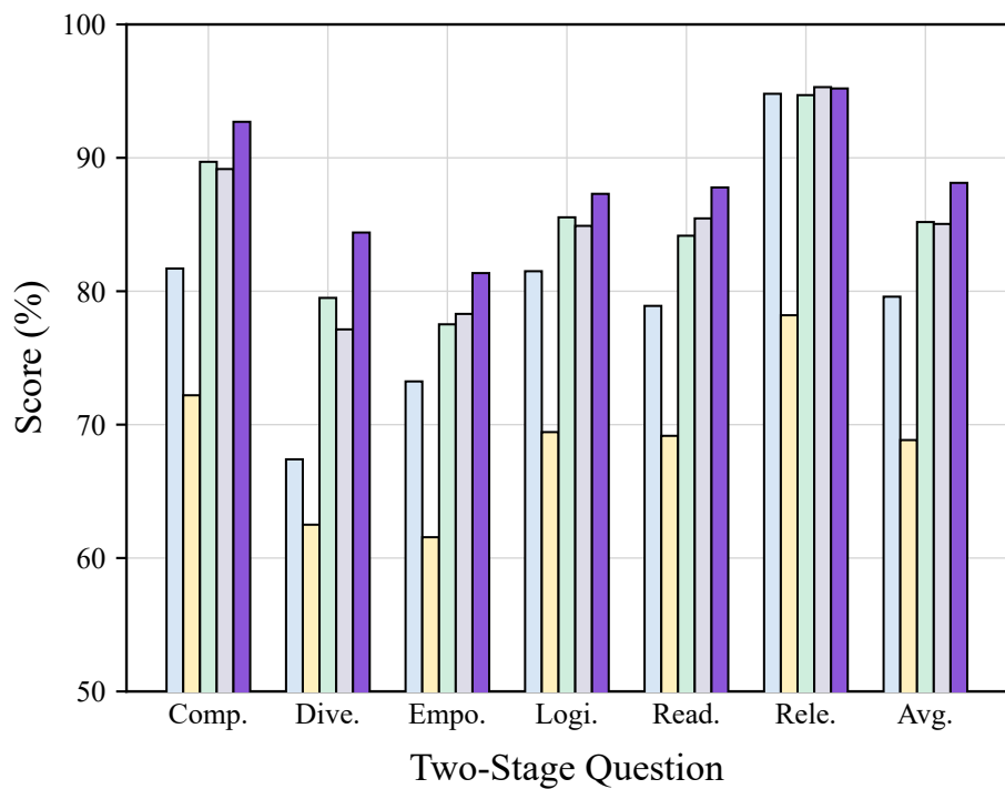
Fig. 5: Experimental results of questions with different difficulty for GPT-4o-mini on the mechanical dataset.
