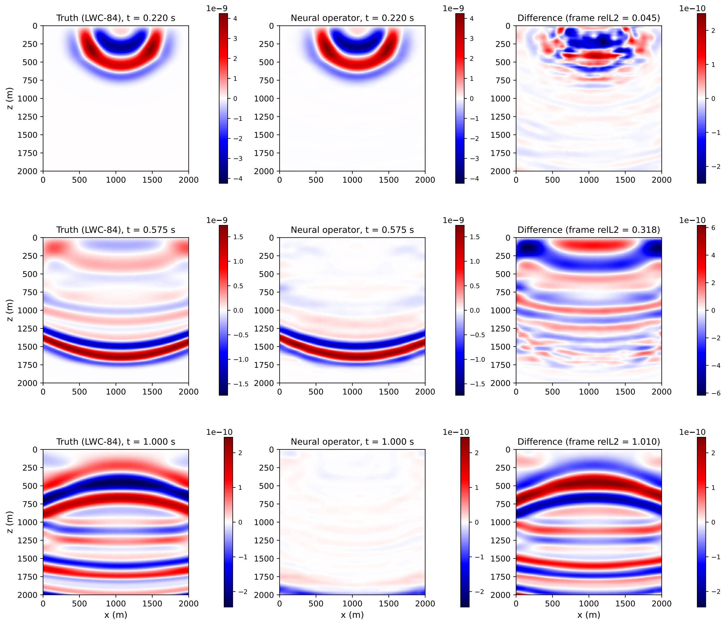
train_layered_00299: truth vs neural operator, early/middle/late (future window starts t = 0.152 s)
