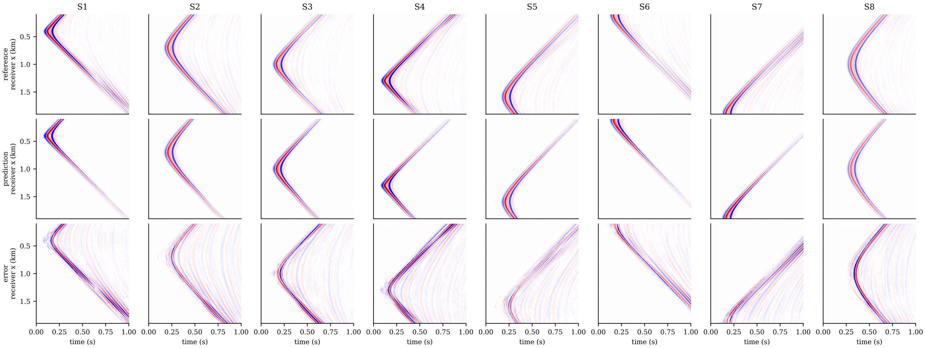
Shallow receiver-line gathers (z=40 m), fixed 19 Hz
