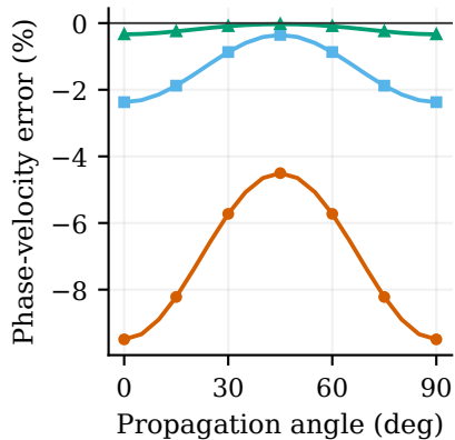
4 points / wavelength
