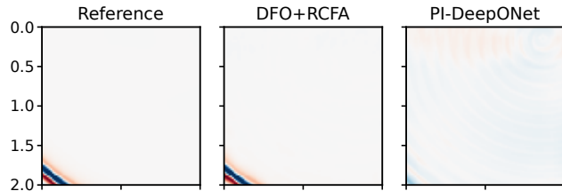
Matched waveform snapshots at t = 0.60 s (train-only development records)
