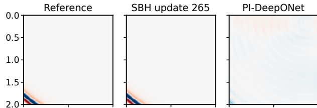
Matched wavefield snapshots at t = 0.60 s (train-development records)
