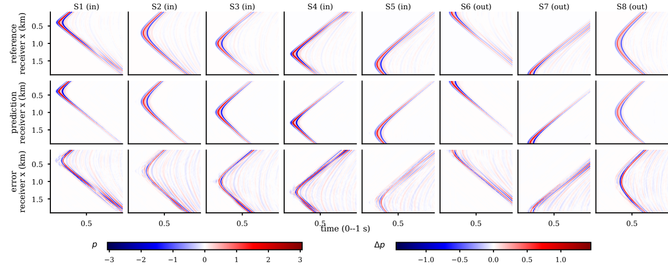
Shallow receiver-line gathers ( z = 40 m), fixed 19 Hz
