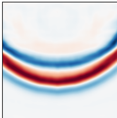
Adapted · t=200
