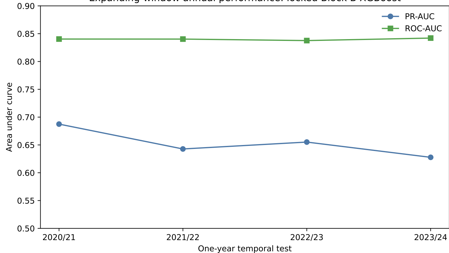
Expanding-window annual performance: locked Block B XGBoost
