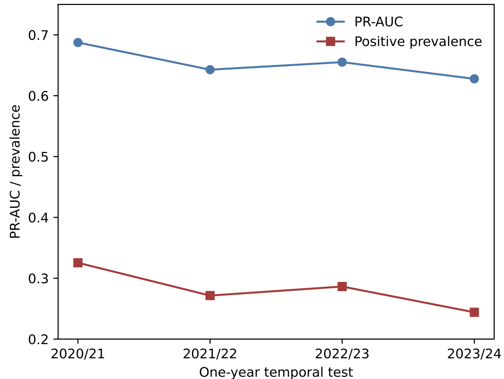
Raw PR-AUC and its prevalence baseline
