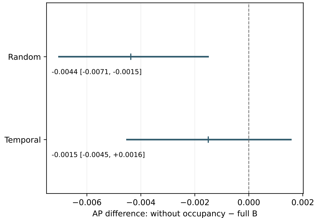
Paired differences on identical test records
