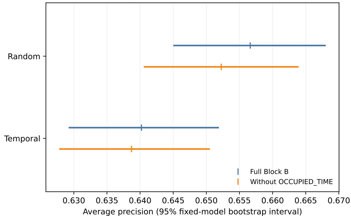
Same split and selected XGBoost settings
