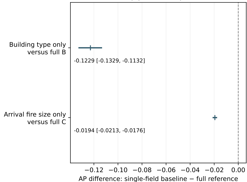
Paired pipeline comparisons
