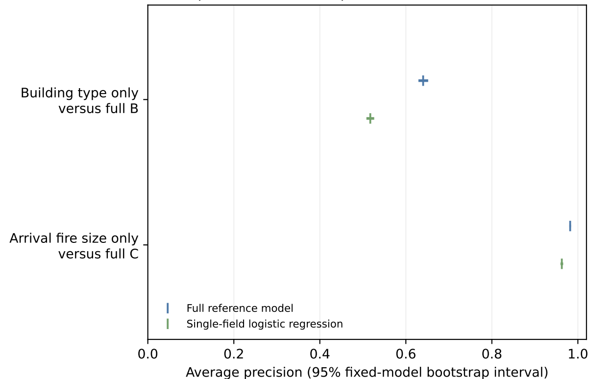
Temporal holdout: simple baselines and full models
