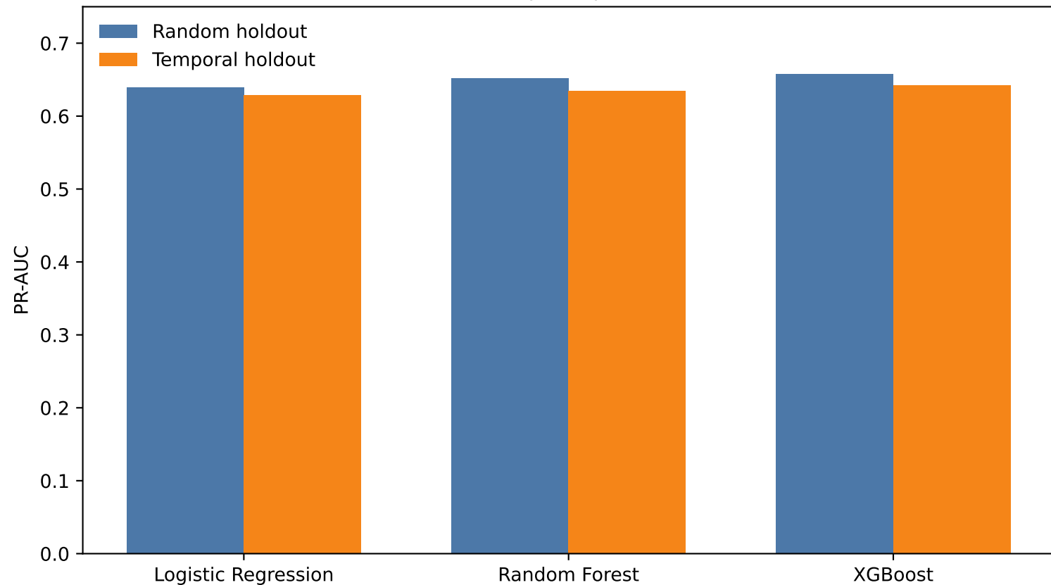
Random versus temporal performance: Block B
