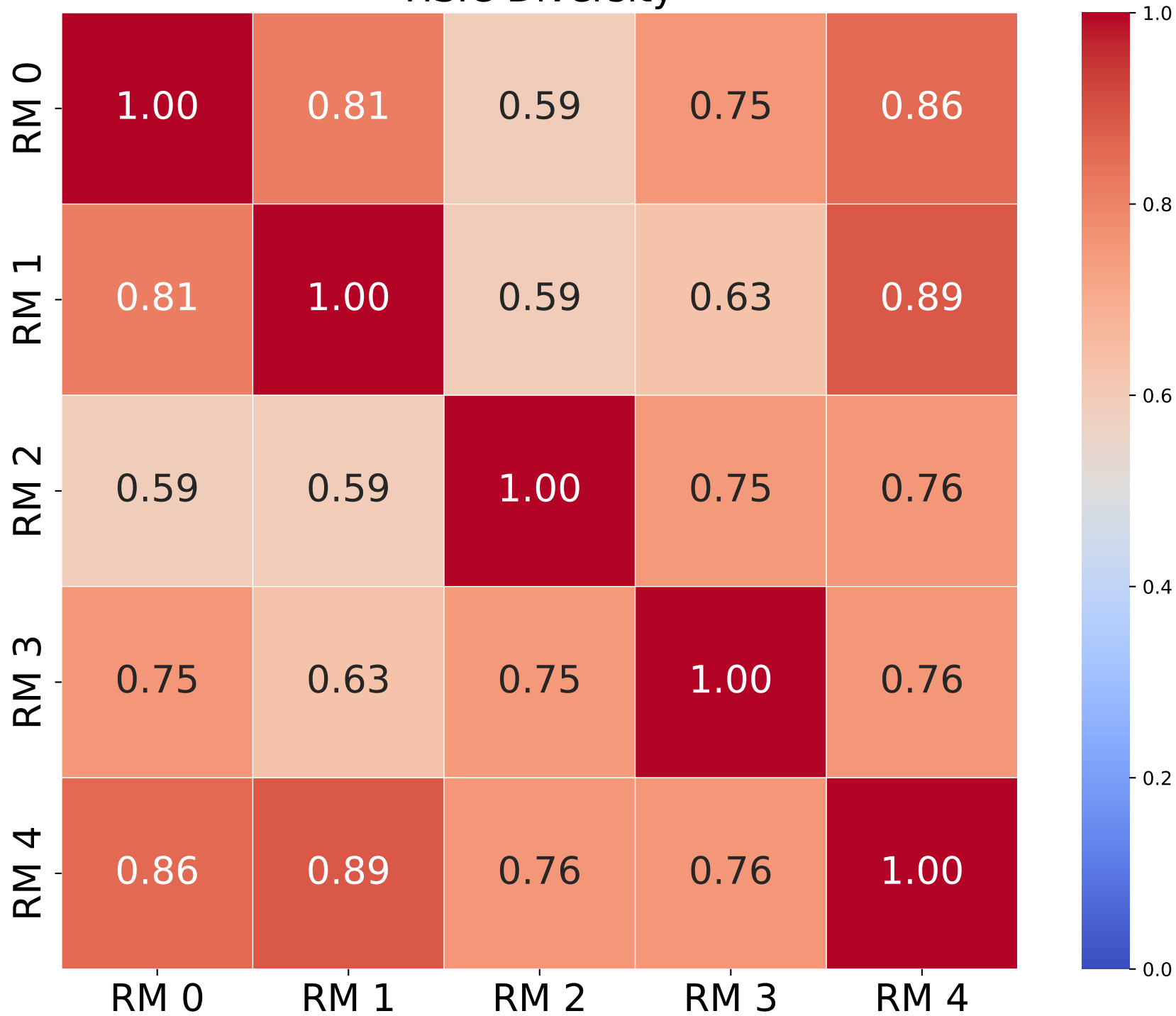
HSIC Diversity
