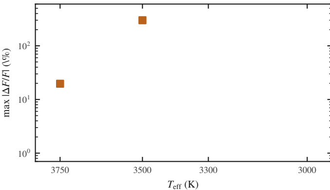
(c) retained M-dwarf atmospheres
