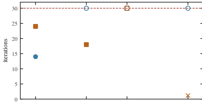
(a) M dwarfs ( \log g = 5.0 )
