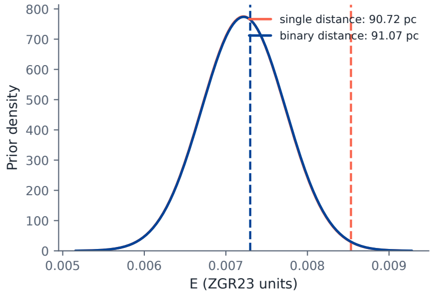
Dust prior at fitted distances
