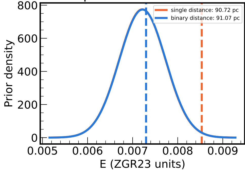
Dust prior at fitted distances
