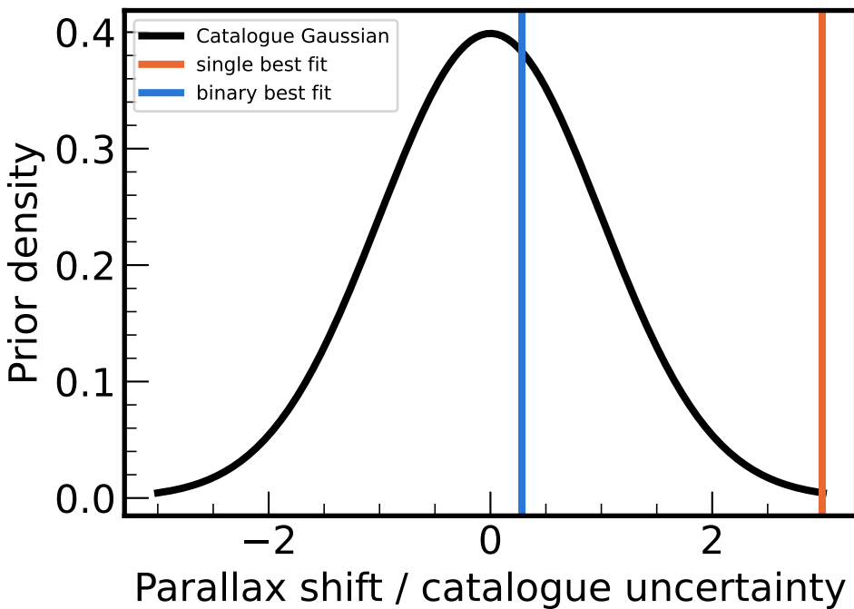
Parallax constraint
