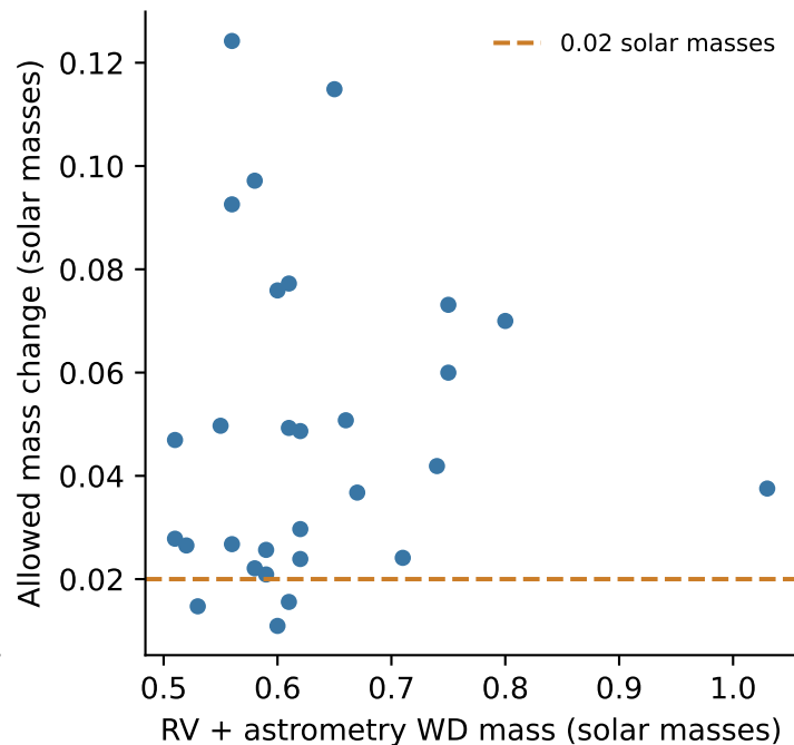
29 Gaia/RV orbits, XP + 2MASS
