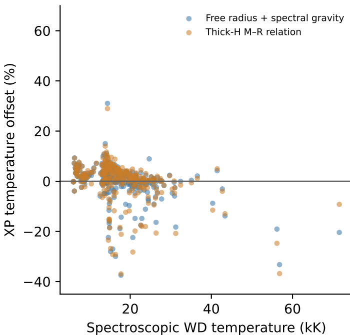
123 spectral decompositions
