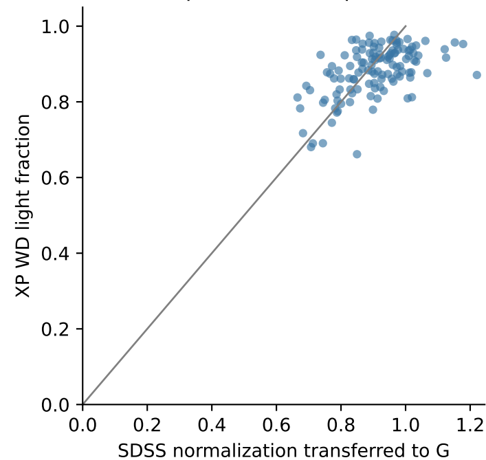
123 spectral decompositions
