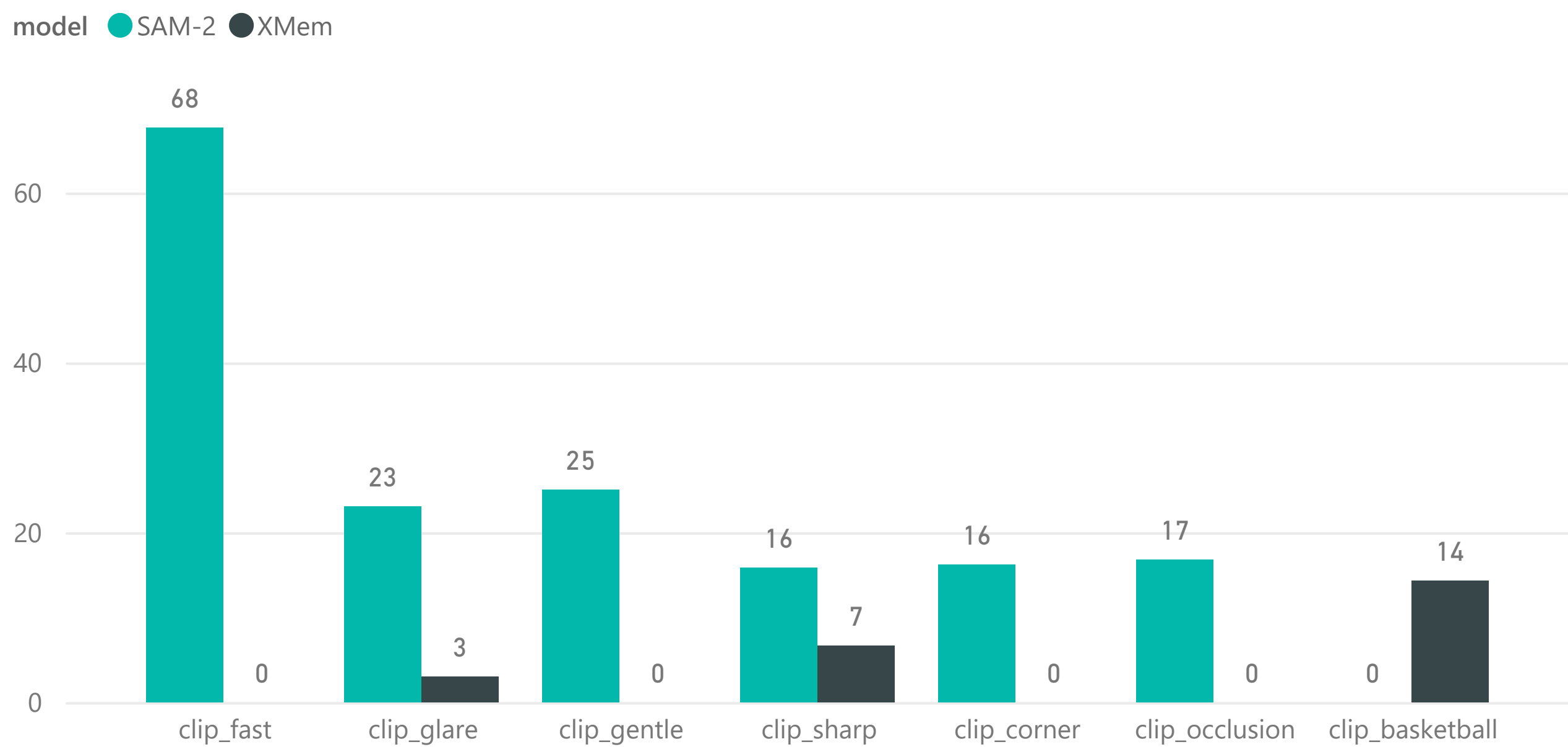
Average of empty_frames_pct by clip_id and m...
