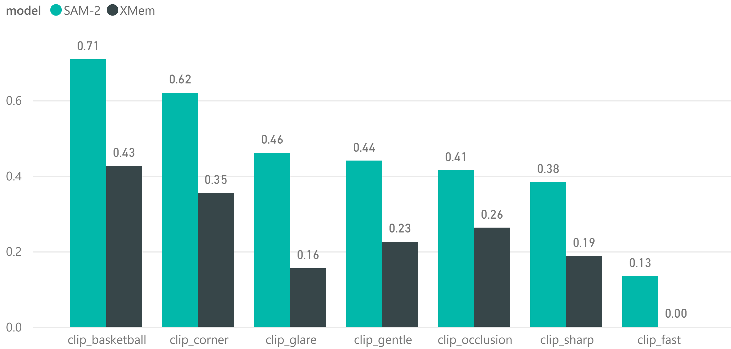
Average of empty_frames_pct by clip_id and m...
