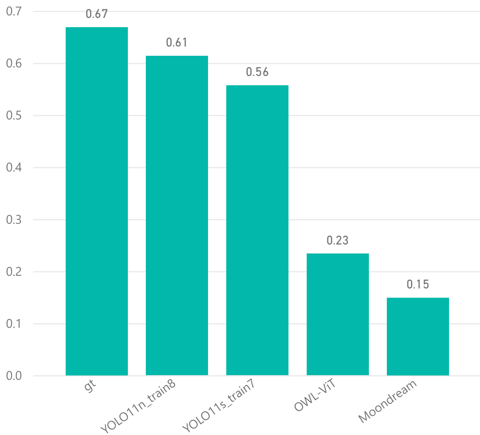
Average of iou_median by (re)prompt...
