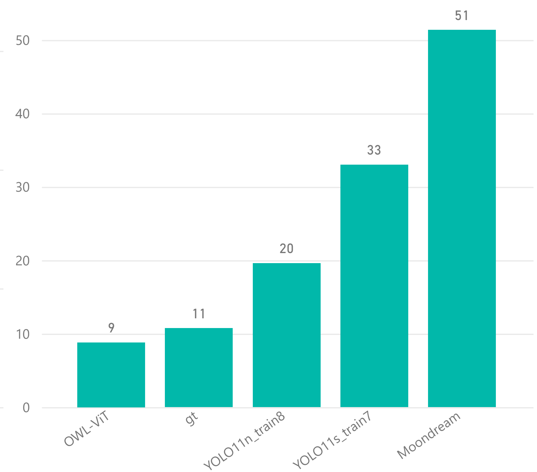
Average of empty_frames_pct by (re)...
