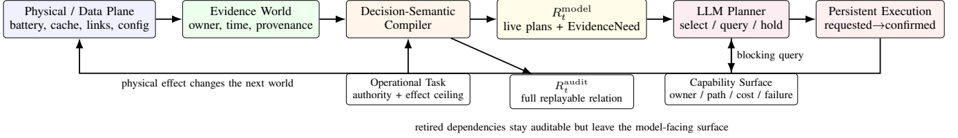
Fig. 1. Closed-loop decision-semantic compilation. The compiler does not recover complete world state. It maintains a typed relation between currently legal plans and their supporting/blocking evidence. A sufficient relation produces a persistent semantic commitment; a blocked relation produces an owner-scoped query whose result re-enters the same compiler.
