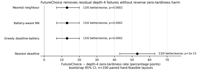
Fig. 4. Paired zero-tardiness gain of FUTURECHOICE over depth-4 receding planning on 100 preselected hard-feasible N=10 layouts. Error bars are paired bootstrap 95% confidence intervals; annotations show favorable/adverse discordance and exact McNemar tests.
