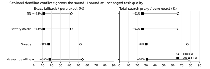
Fig. 5. B→C attribution. The deadline-set MST bound reduces exact fallback and total exact-correct search work relative to the earlier basic optimistic bound at unchanged task quality.
